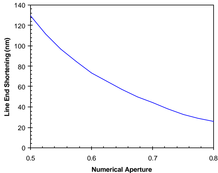
Figure 8. Larger numerical apertures reduce the loss of image fidelity due to diffraction, producing less line end shortening (180nm line, \lambda = 248\text{nm} , \sigma = 0.5 ).
