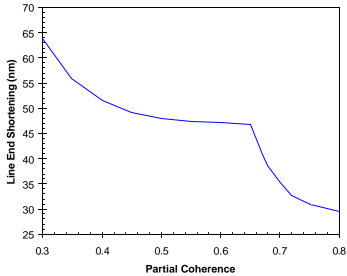
Figure 9. Partial coherence shows a somewhat discontinuous impact on the aerial image line end shortening (180nm line, \lambda = 248\text{nm} , \text{NA} = 0.688 ).
