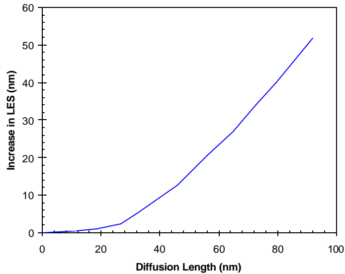
Figure 10. Diffusion can have a dramatic effect on line end shortening (180nm line, \lambda = 248\text{nm} , \text{NA} = 0.688 , \sigma = 0.5 ).
