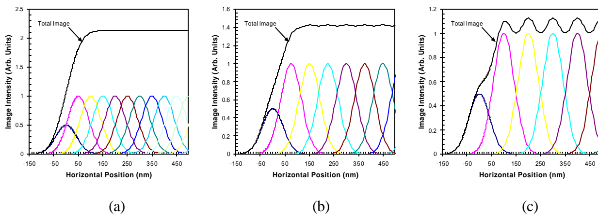
Figure 2. Example summations of 100nm Gaussian spots for physical address grids of (a) 50nm, (b) 75nm, and (c) 100nm. In this case, the edge pixel is set to 50% gray level.
